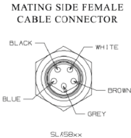
Figure 4-7: M8 Female Mating Cable Connector Pin
