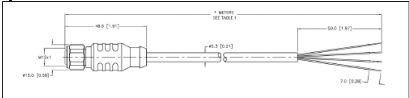
Figure 4-8 M12 Power Cable
